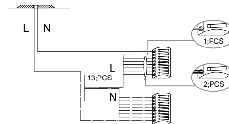
MAPA ROSONE LED CLOUD SP25 - schema cablaggio / wiring diagram
