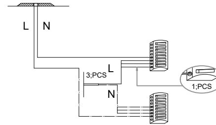
MAPA ROSONE LED CLOUD SP7 - schema cablaggio / wiring diagram
