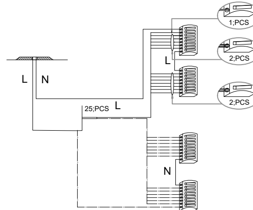
MAPA ROSONE LED CLOUD SP25 - schema cablaggio / wiring diagram
